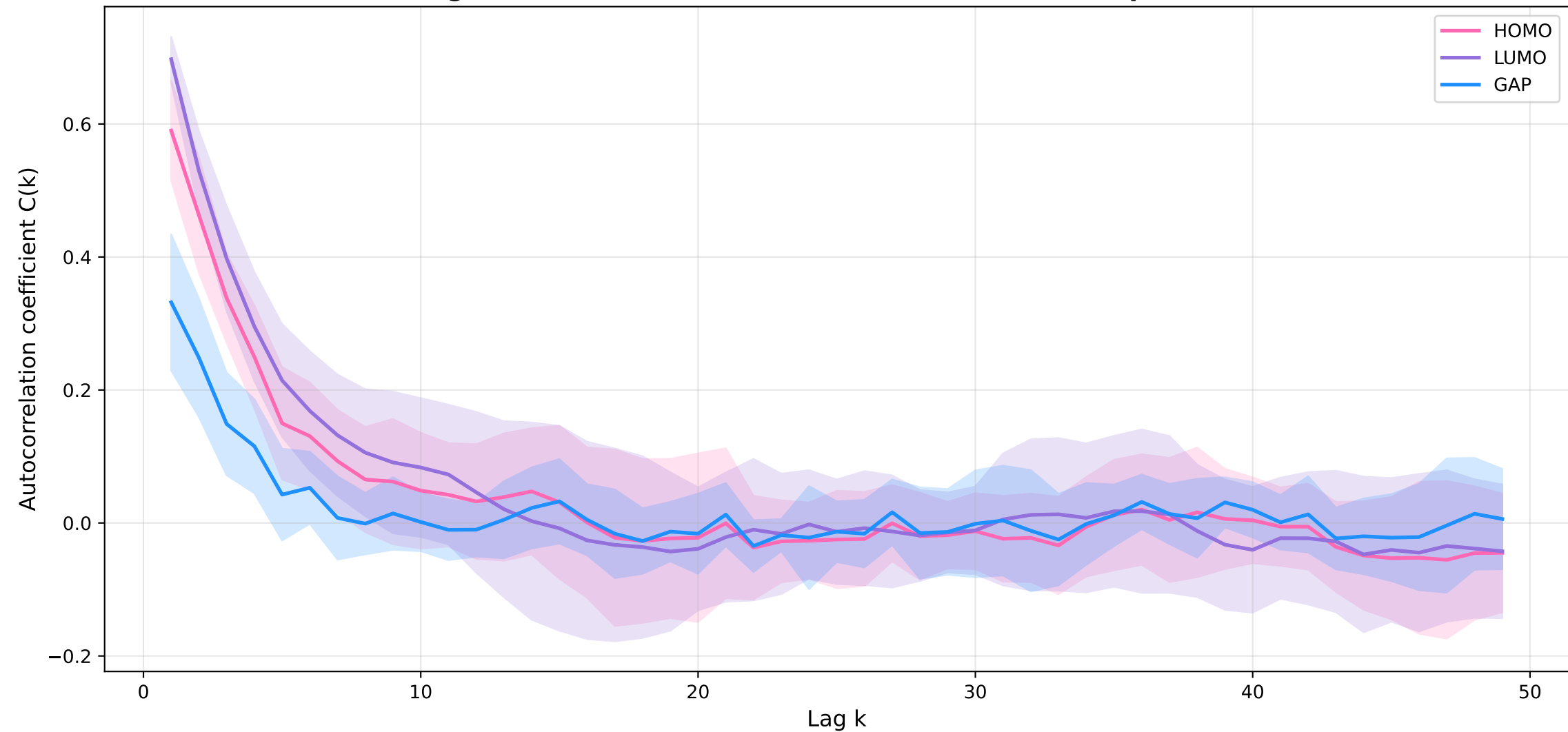
Average autocorrelations (HOMO, LUMO, GAP) for Experiment 2D
