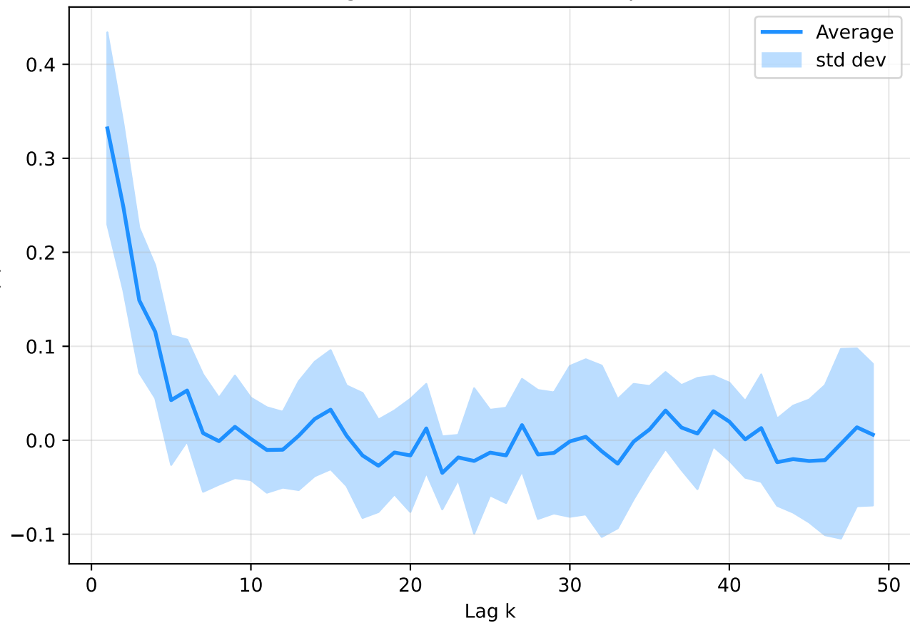
GAP - Average autocorrelation for Experiment 2D
