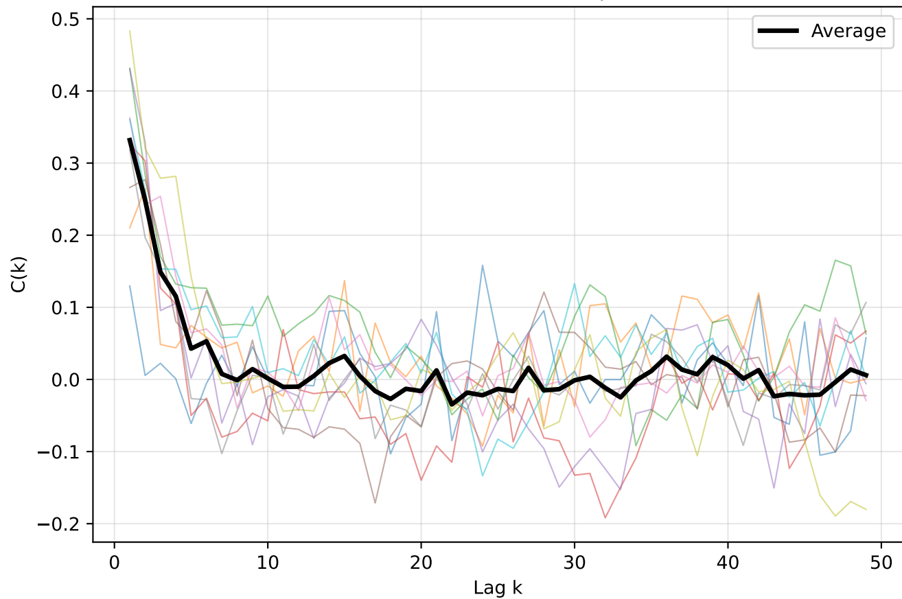
GAP - All autocorrelation for Experiment 2D
