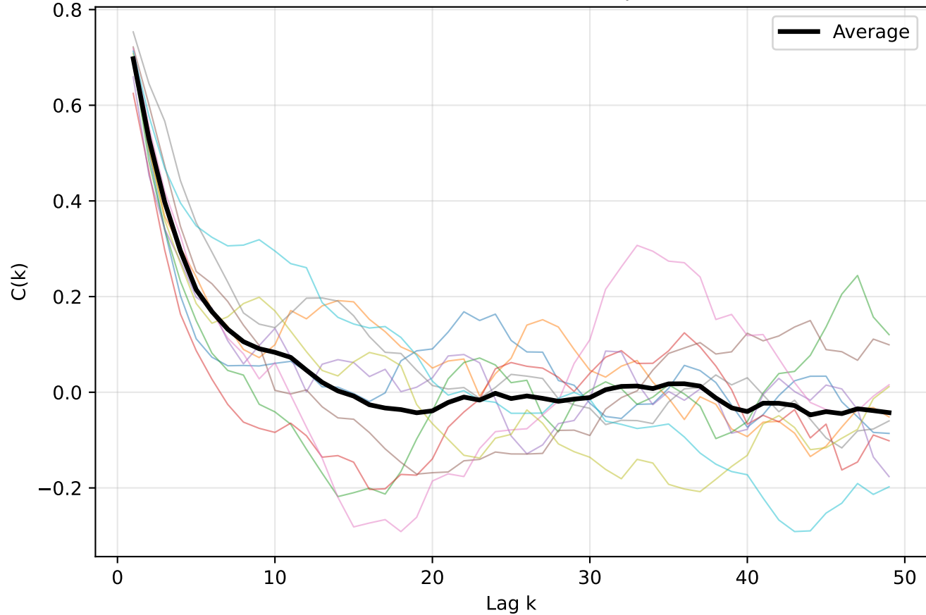
LUMO - All autocorrelation for Experiment 2D
