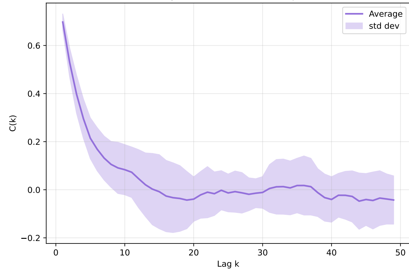
LUMO - Average autocorrelation for Experiment 2D
