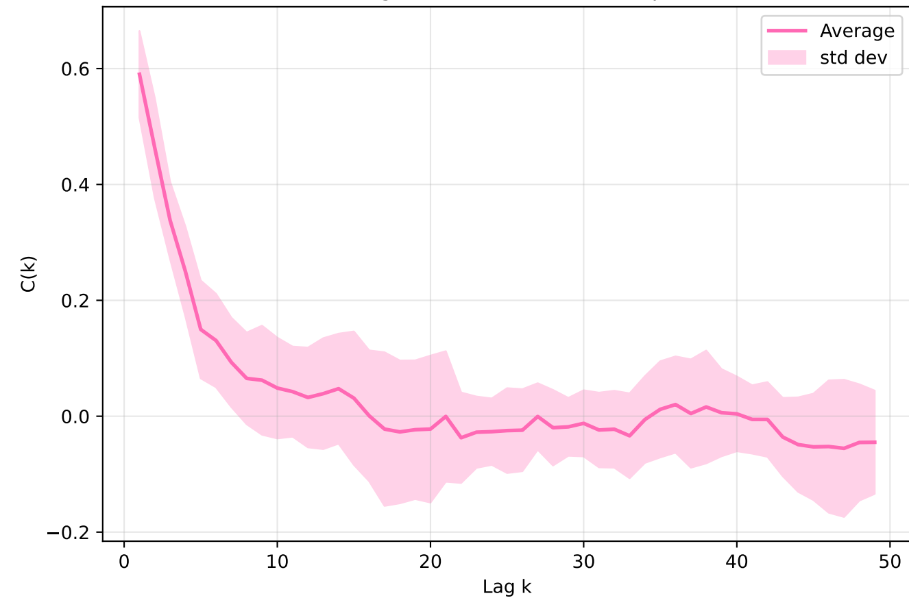
HOMO - Average autocorrelation for Experiment 2D
